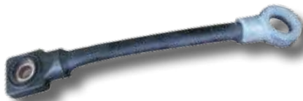
BAT/18358 Flexible welded connections: 1 x welded and 1 x screwed
